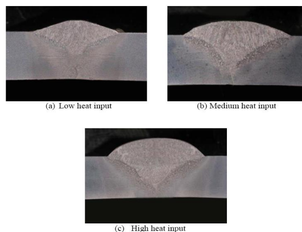
Figure-2. Macrograph of weld specimen at the different heat input.
